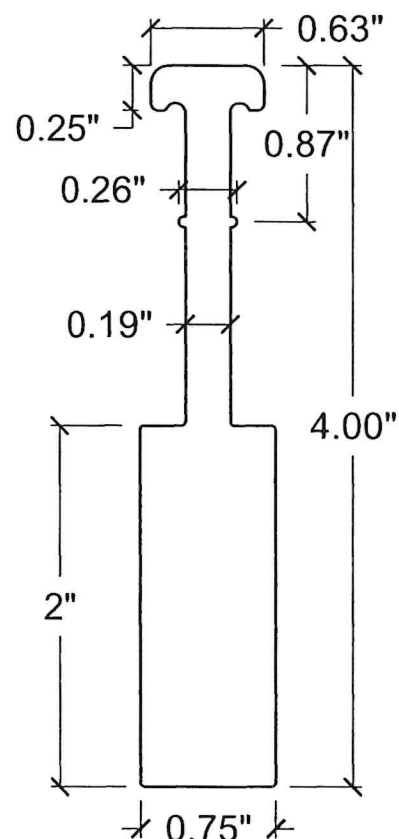
END RETENTION "T" BAR (3/16" THICK) CAST ALUM.
