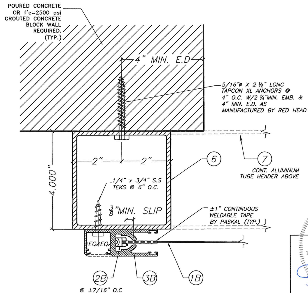
SECTION F-F: BUILD-OUT MOUNTED (PLAN)* SCALE: N.T.S.
