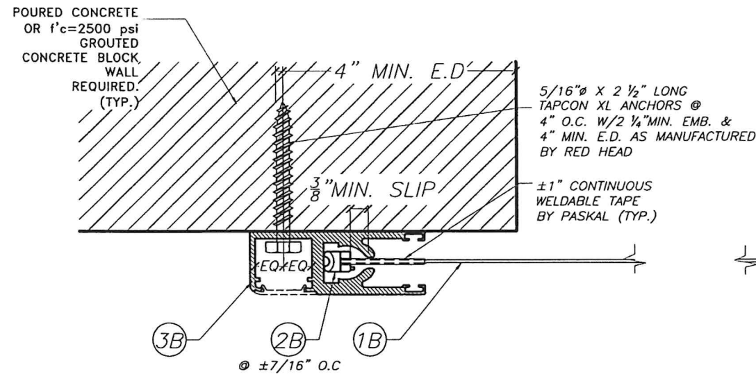
SECTION B-B: WALL MOUNTED (PLAN)* SCALE: N.T.S.
