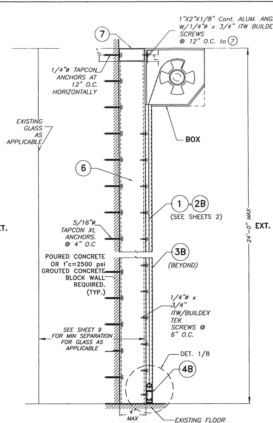
SECTION E-E BUILD OUT MOUNTED SCALE N.T.S.
