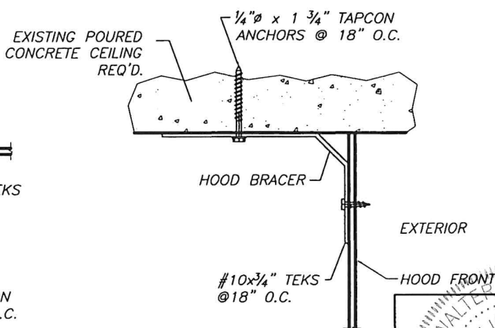
CEILING HOOD ATTACHMENT (SIDE VIEW)
