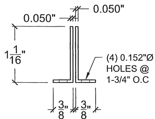
END RETENTION ANGLES (LENGTH 2 3/4") 3105-H14 ALUM. ALLOY
