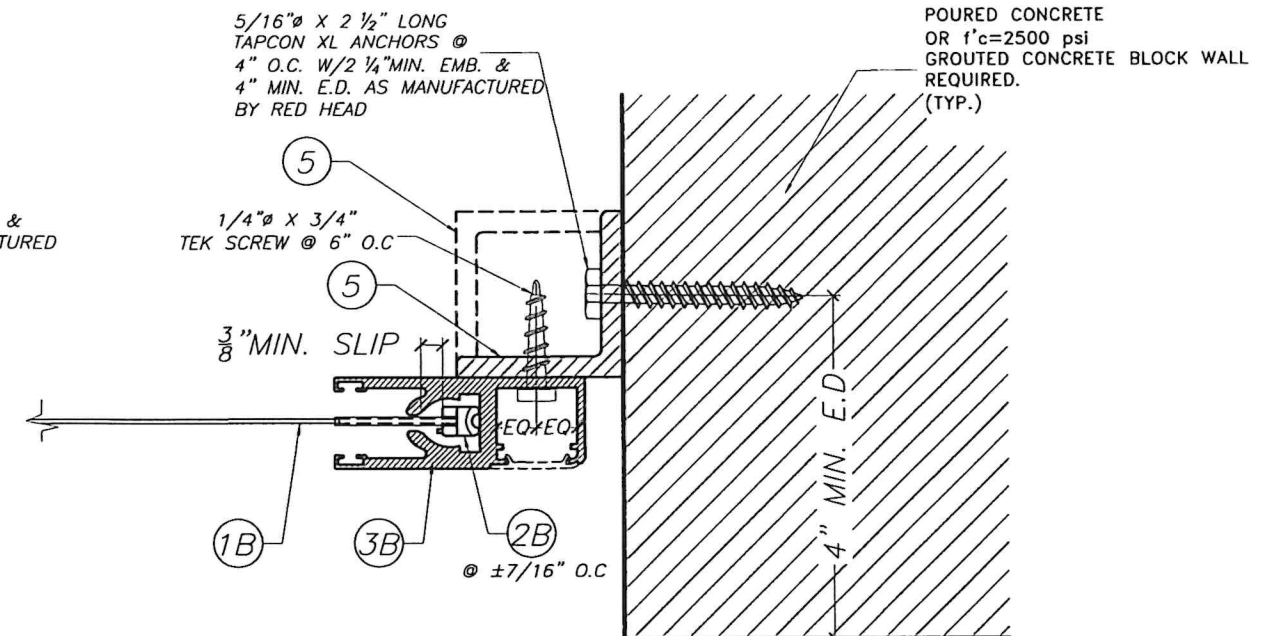
SECTION D-D: TRAPPED MOUNTED (PLAN)* SCALE: N.T.S.
