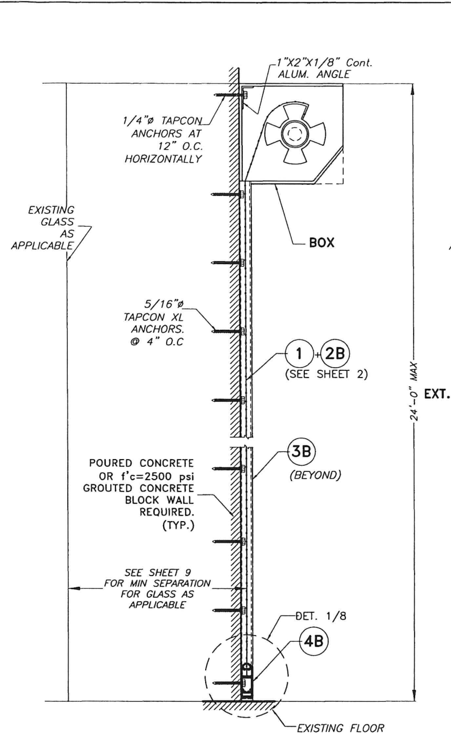
SECTION A-A WALL MOUNTED SCALE N.T.S.
